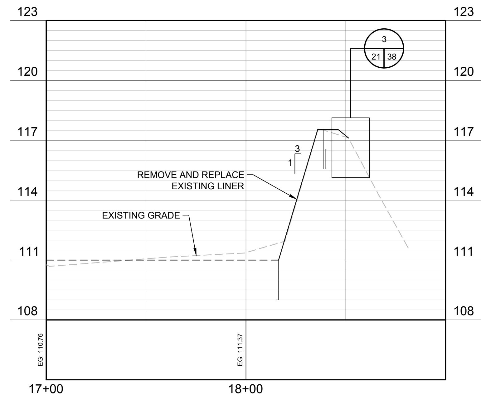
RIBS 2-4 SECTION
