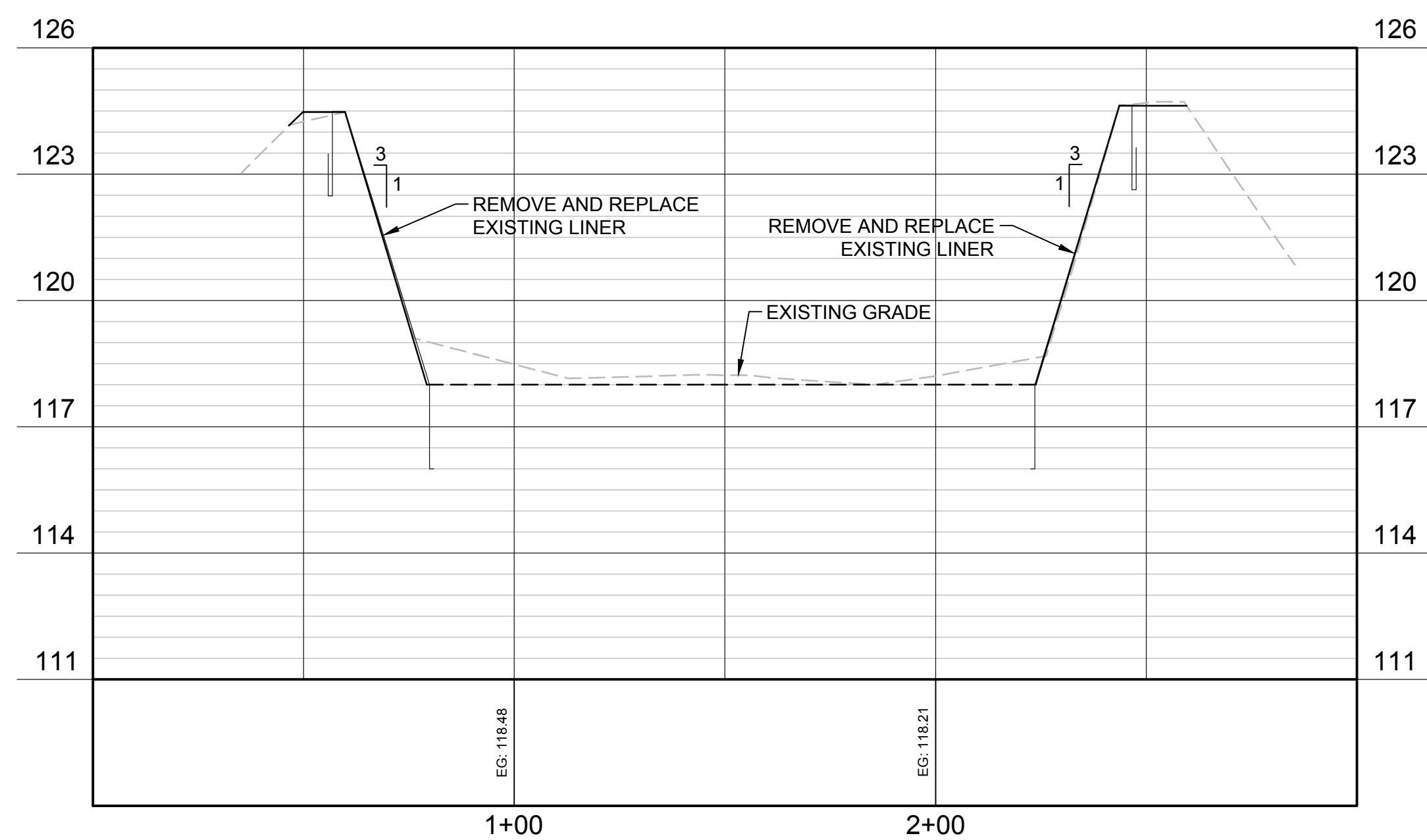
RIBS 3 SECTION
