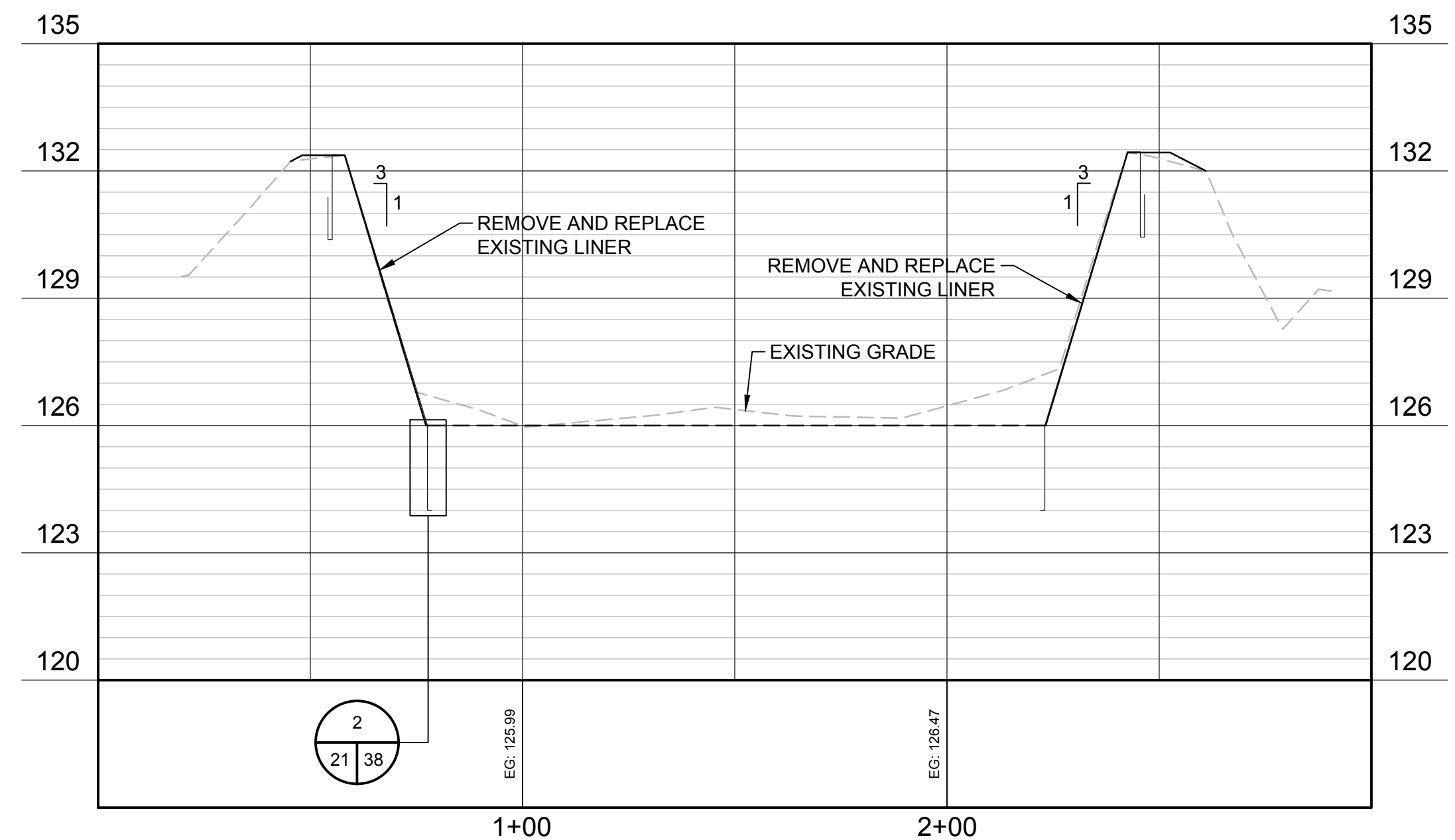
RIBS 2 SECTION
