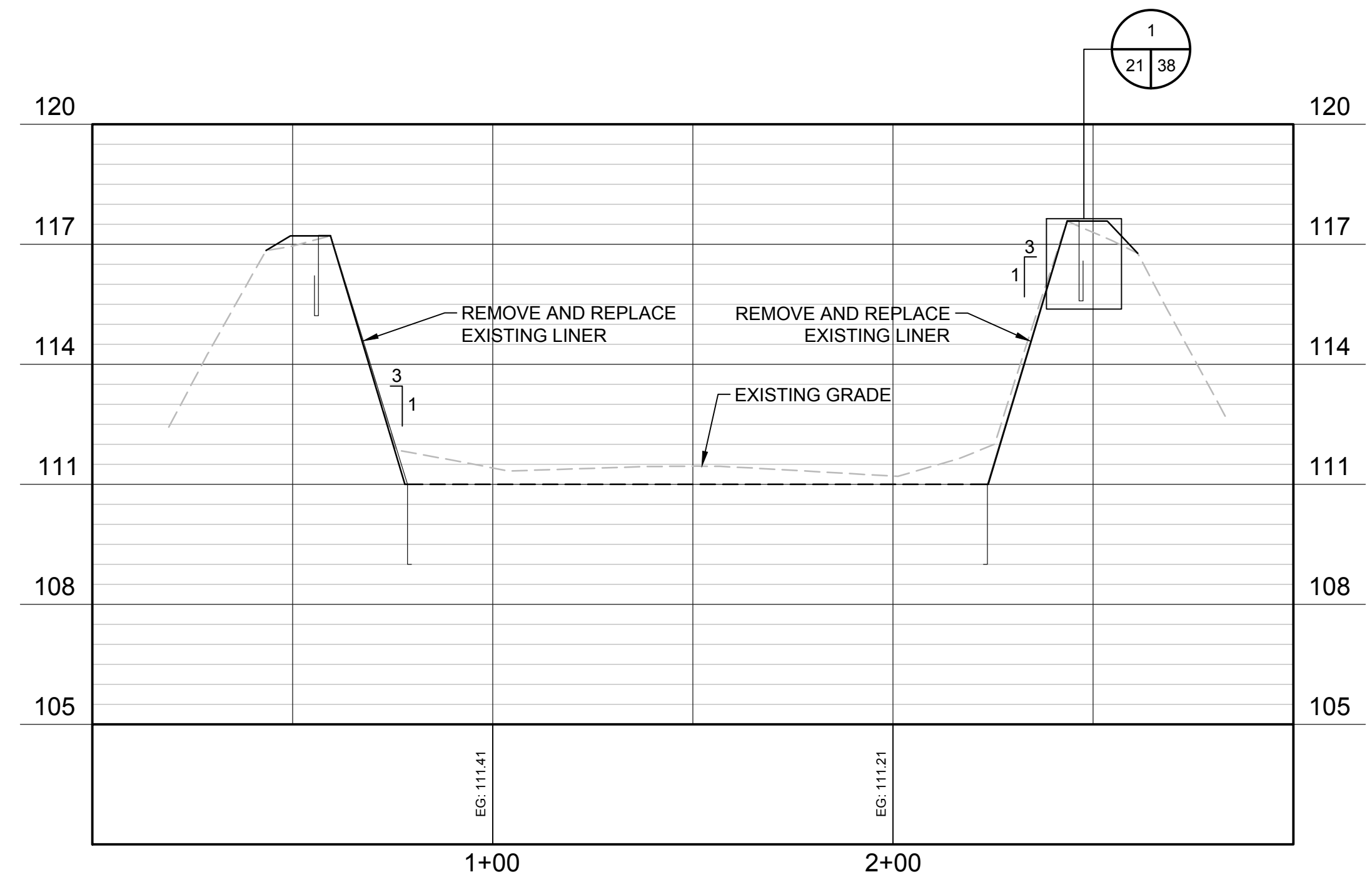
RIBS 4 SECTION
