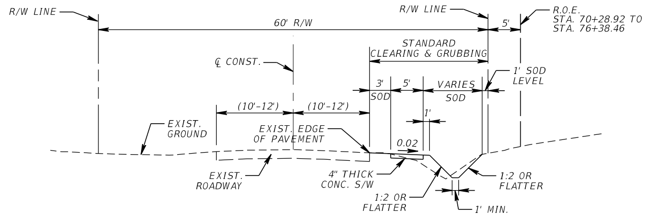
TYPICAL SECTION 6 COLLEGE DR. STA. 70+00.00 TO STA. 76+50.00
