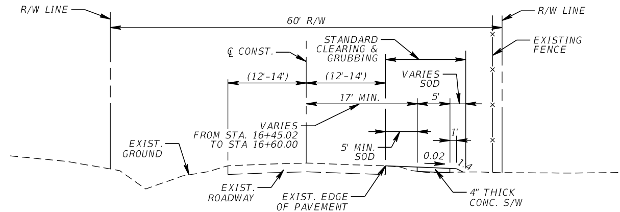
TYPICAL SECTION 8 COLLIER BLVD. STA. 15+50.00 TO STA. 16+60.00
