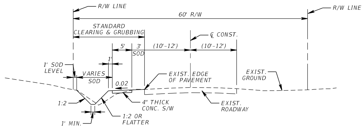
TYPICAL SECTION 2
