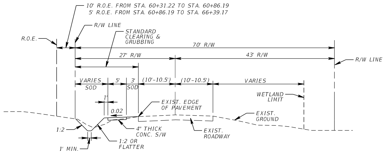
TYPICAL SECTION 7 CARTER ST. STA. 60+00.00 TO STA. 66+50.00
