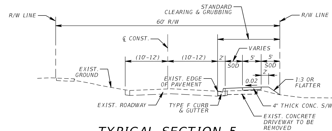
TYPICAL SECTION 5
