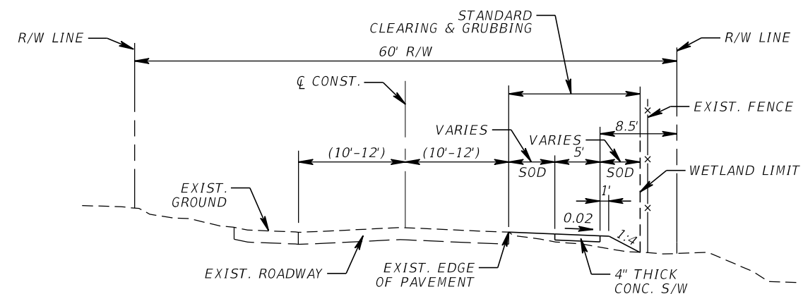
TYPICAL SECTION 4
