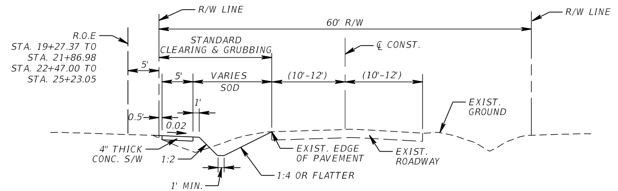
TYPICAL SECTION 3
