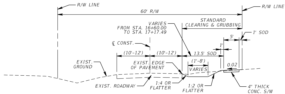
TYPICAL SECTION 1
