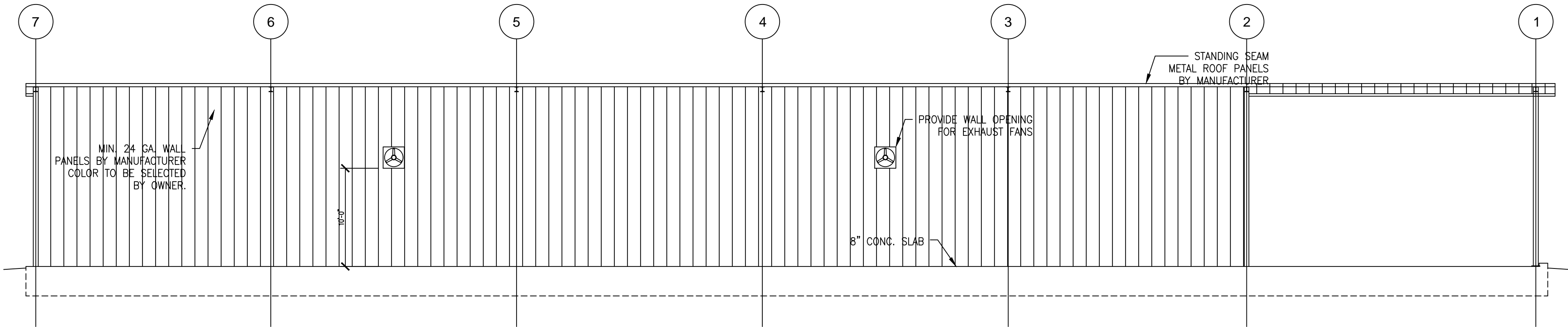
3 SOUTH ELEVATION SCALE: 3/16" = 1'-0"
