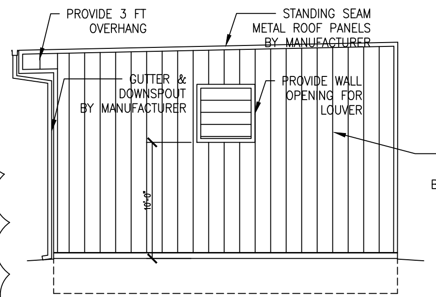
2 WEST ELEVATION SCALE: 3/16" = 1'-0"
