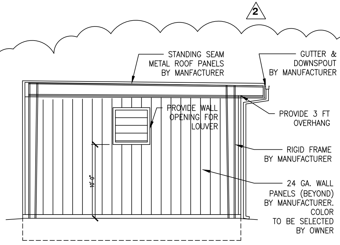
4 EAST ELEVATION SCALE: 3/16" = 1'-0"
