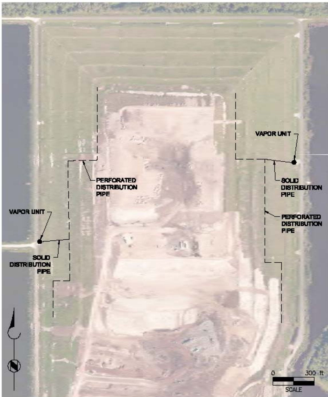
FIGURE 1 ODOR CONTROL SYSTEM LAYOUT FOR TWO NEW UNITS ORANGE COUNTY SOLID WASTE MANAGEMENT FACILITY- CELL 9-12
